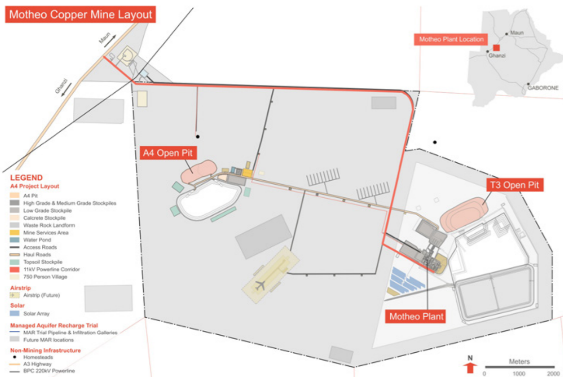
Motheo Copper Mine showing the planned integration of the A4 Deposit as part of an expanded 5.2Mtpa production hub.
